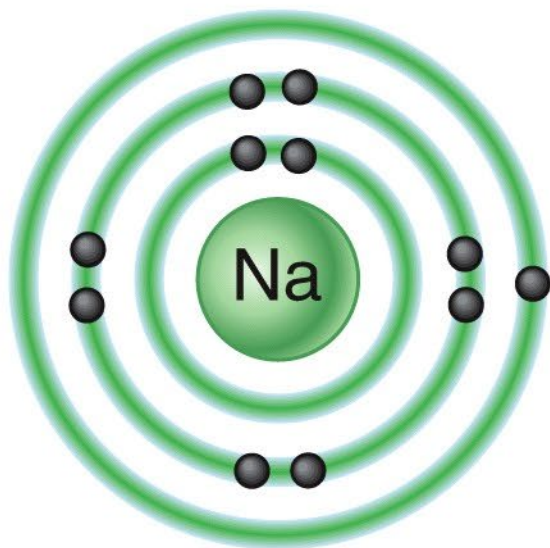
Atom
